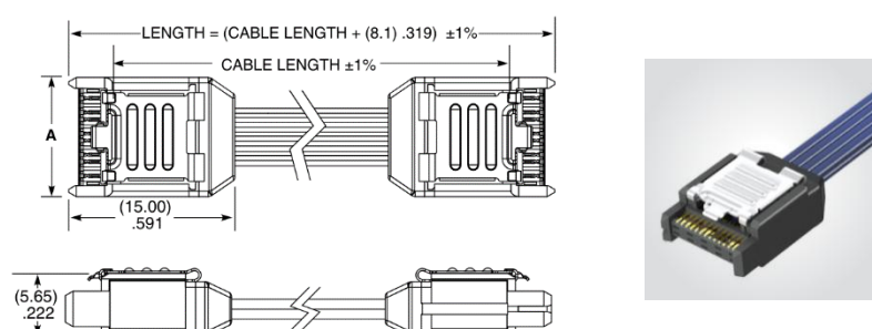
Figure 4: High-speed ARC6-08 cable
