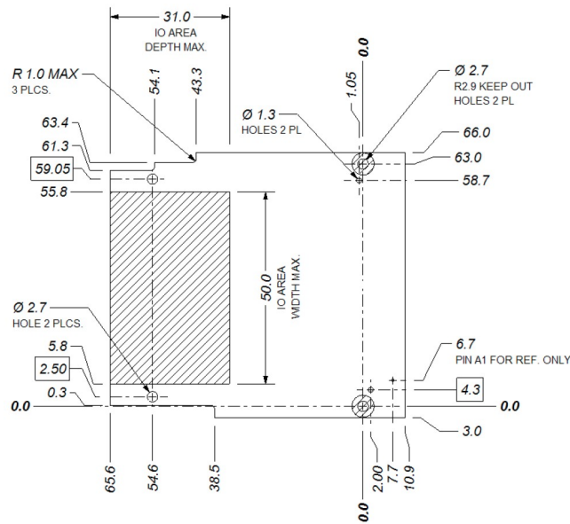
Figure 2: PCB dimensions (all dimensions in mm)
